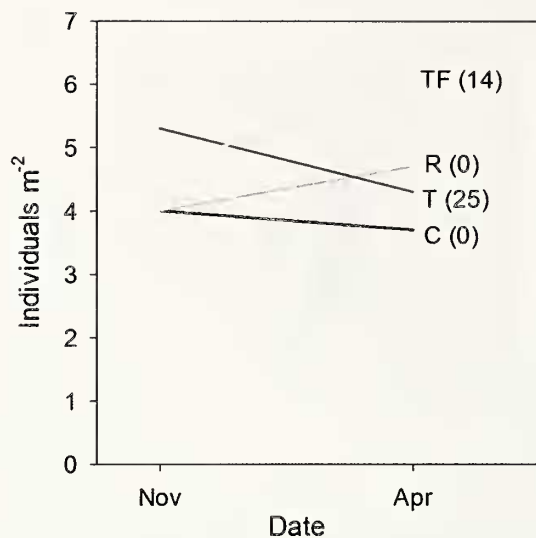
Fig. 4. Mean density of adult/sub-adult dew worms Lumbricus terrestris from a 5 month density manipulation and tagging experiment starting in November and ending in April ( n=3 ). In "R" all individuals obtained in sampling were removed at the start of the experiment, in "C" they were returned to their burrows. In T and TF, sampled individuals were tagged and then returned to burrows, with plots fenced in TF. The values in parentheses give the % of tagged individuals from November sampling.
